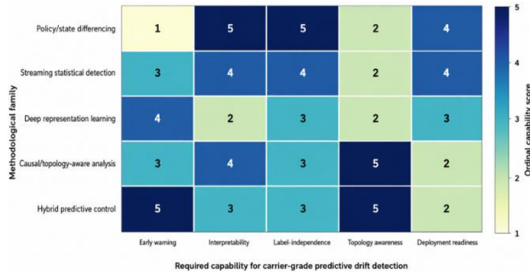
Figure 3: Capability Profile of Methodological Families for Predictive Carrier-Network Drift Detection
