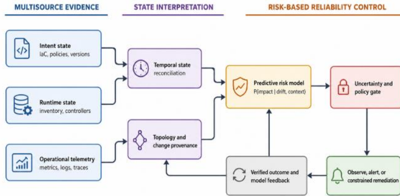
Figure 1: Predictive Infrastructure Drift Detection Framework for Cloud-Native Carrier Reliability
